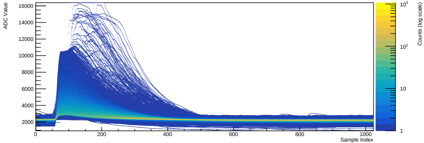
Run 039518 - Channel 2080 (n=38242 waveforms)
