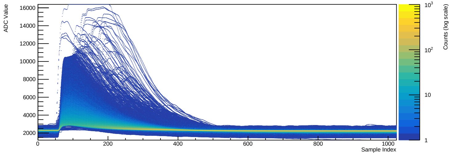
Run 039522 - Channel 2080 (n=35399 waveforms)
