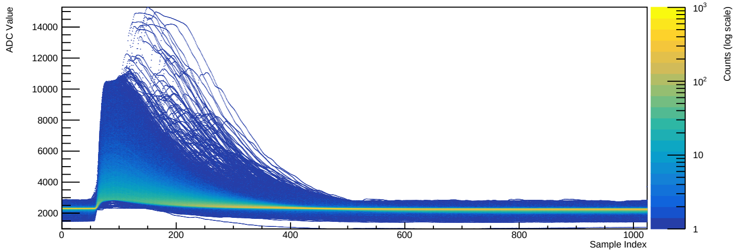
Run 039523 - Channel 2080 (n=34420 waveforms)
