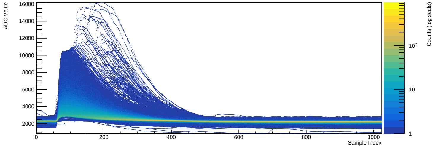
Run 039528 - Channel 2080 (n=32160 waveforms)
