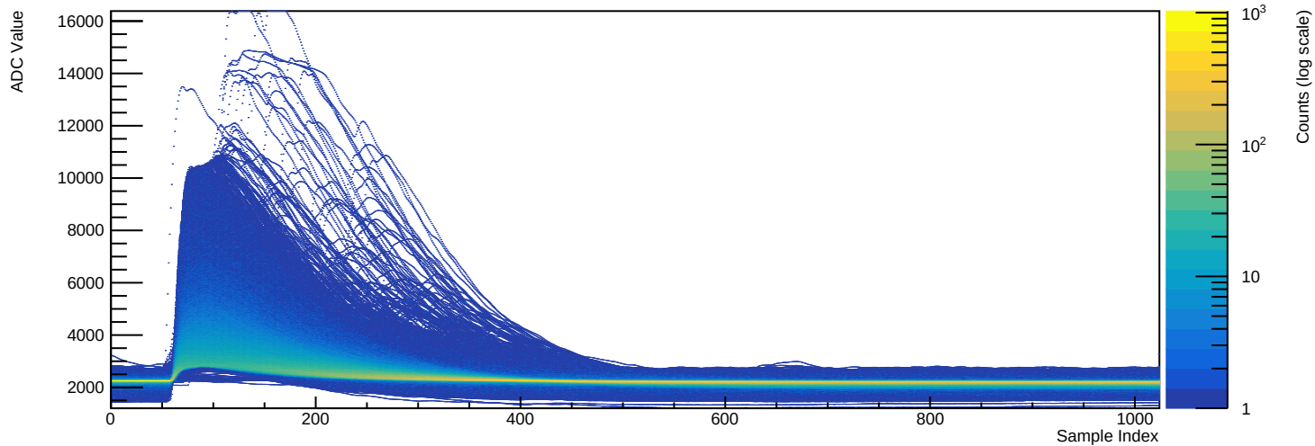
Run 039500 - Channel 2081 (n=31474 waveforms)
