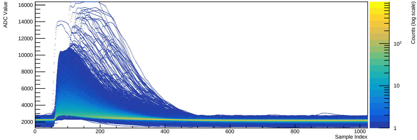
Run 039503 - Channel 2081 (n=35420 waveforms)
