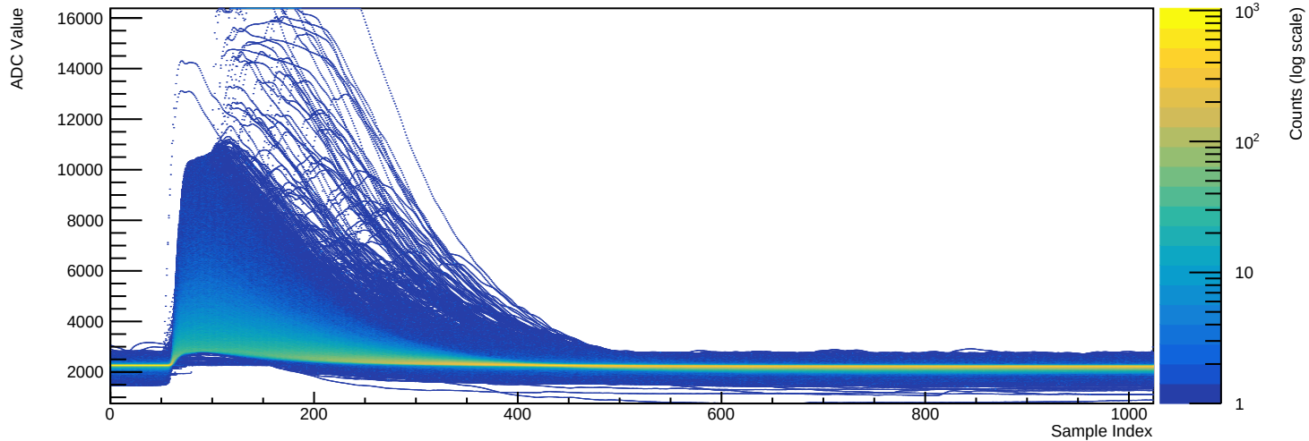
Run 039504 - Channel 2081 (n=36788 waveforms)
