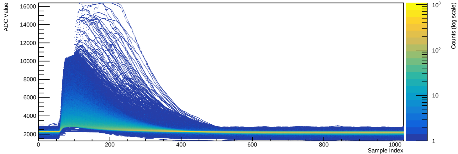
Run 039507 - Channel 2081 (n=41306 waveforms)
