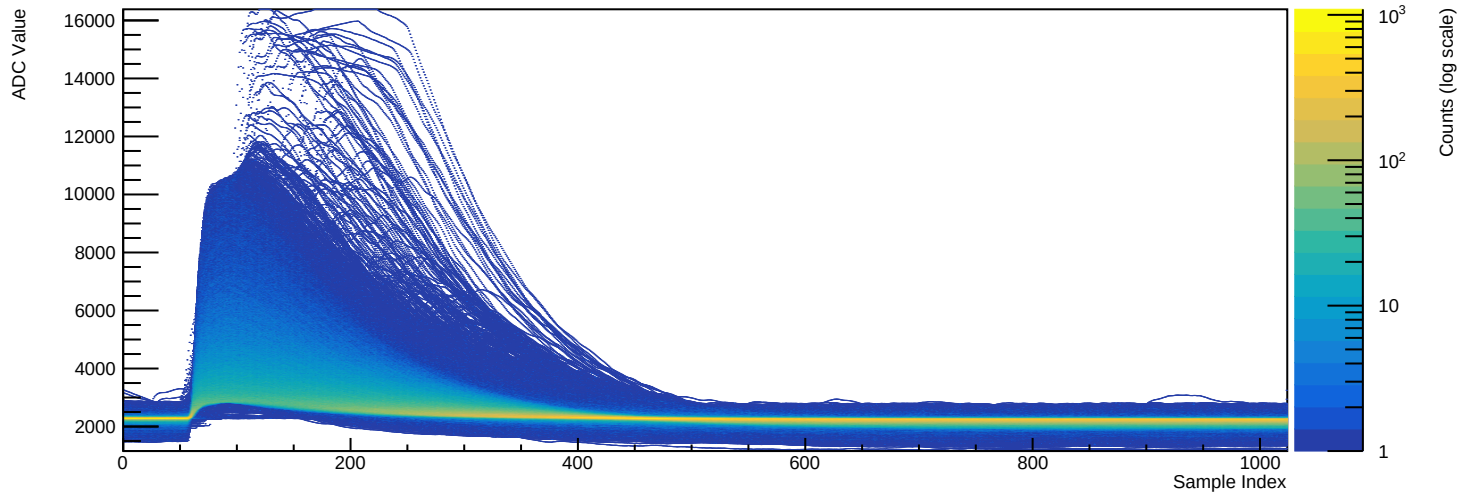
Run 039510 - Channel 2081 (n=47507 waveforms)
