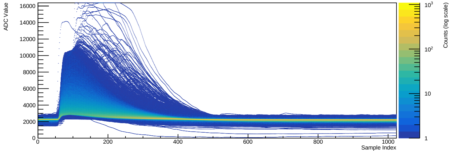
Run 039511 - Channel 2081 (n=46395 waveforms)
