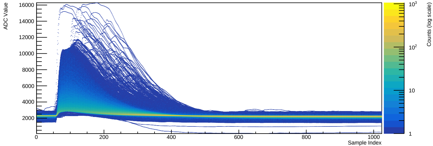
Run 039515 - Channel 2081 (n=39804 waveforms)
