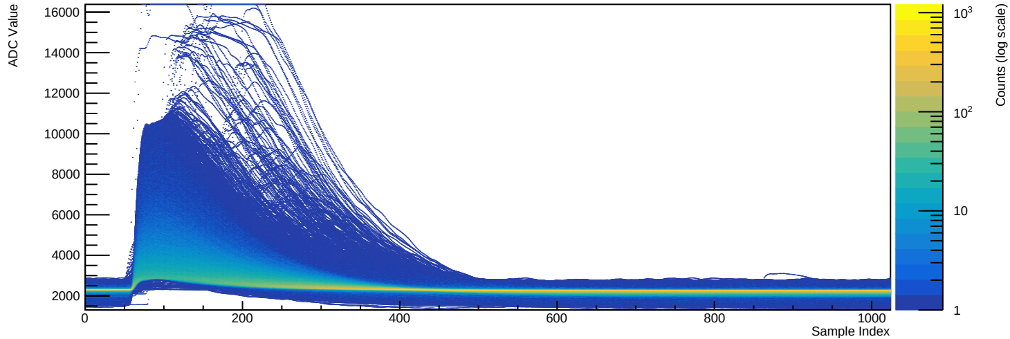
Run 039516 - Channel 2081 (n=38693 waveforms)
