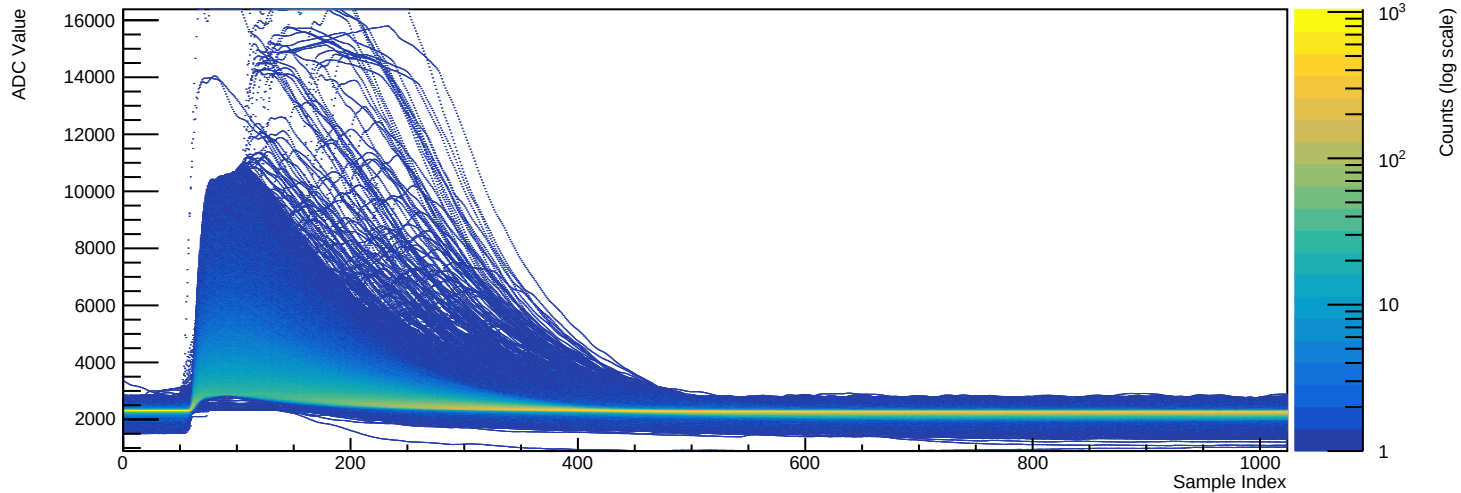
Run 039519 - Channel 2081 (n=36497 waveforms)
