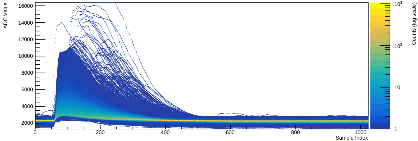
Run 039521 - Channel 2081 (n=35297 waveforms)
