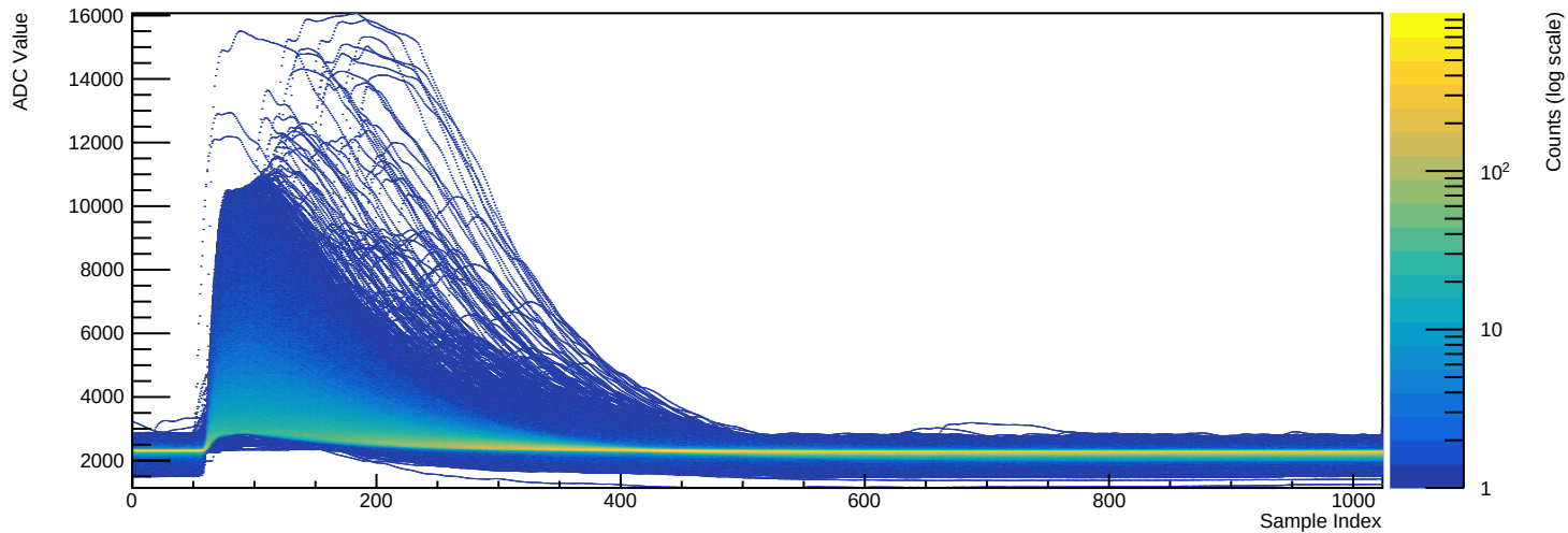
Run 039522 - Channel 2081 (n=34830 waveforms)
