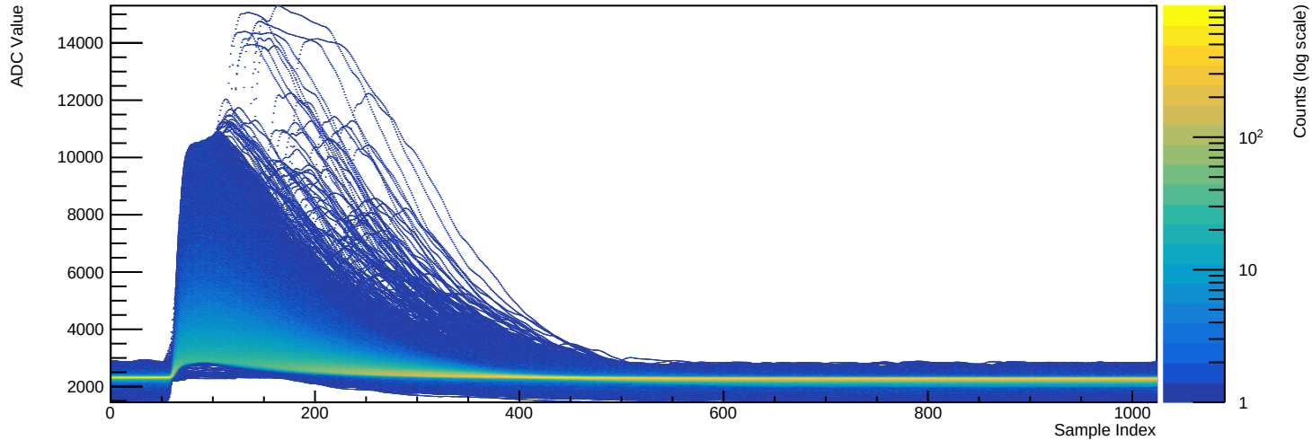
Run 039523 - Channel 2081 (n=33759 waveforms)
