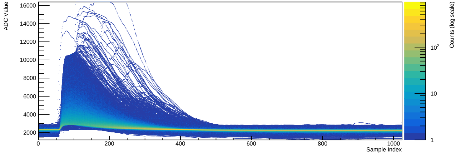
Run 039526 - Channel 2081 (n=32484 waveforms)
