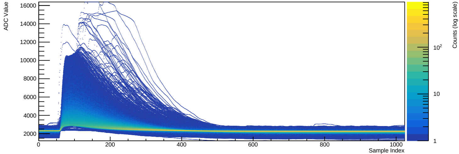
Run 039527 - Channel 2081 (n=32008 waveforms)
