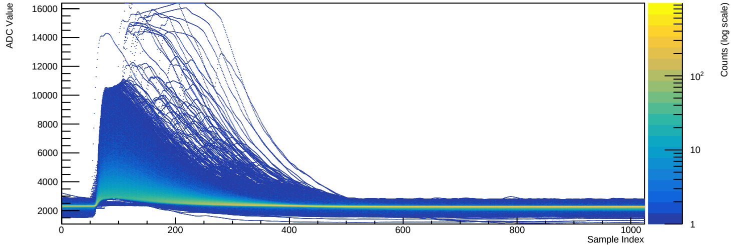
Run 039529 - Channel 2081 (n=30916 waveforms)
