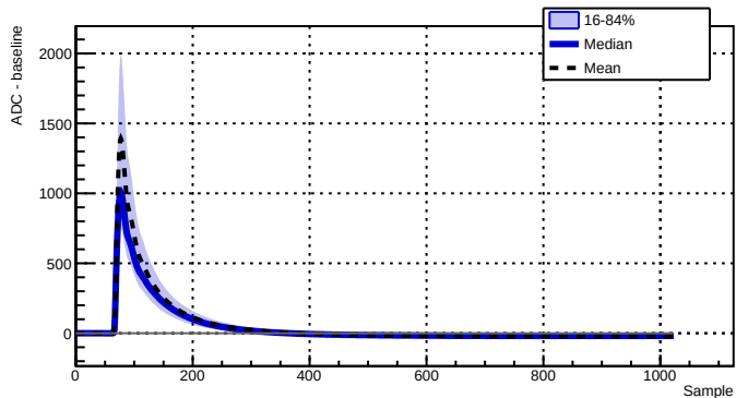
Run 039500 - Channel 2070 - 9421 waveforms
