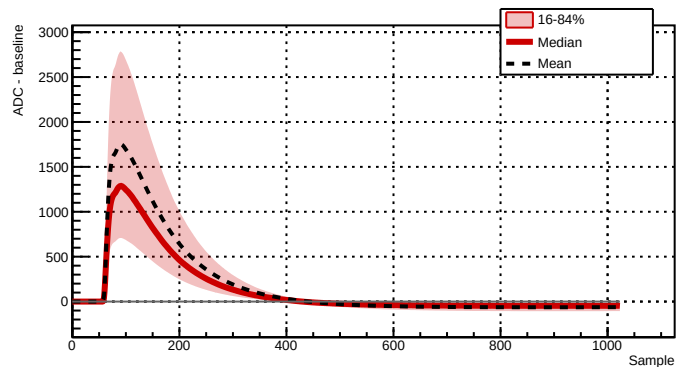
Run 039500 - Channel 2081 - 31474 waveforms
