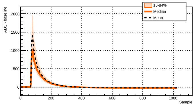
Run 039500 - Channel 2071 - 8959 waveforms
