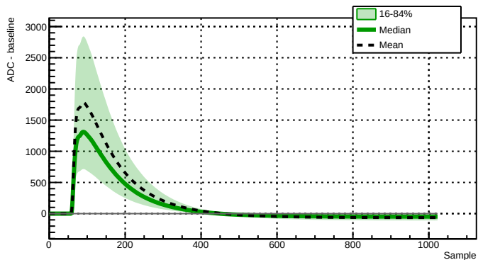
Run 039500 - Channel 2080 - 32054 waveforms
