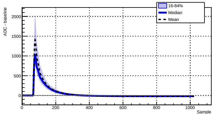
Run 039501 - Channel 2070 - 9678 waveforms
