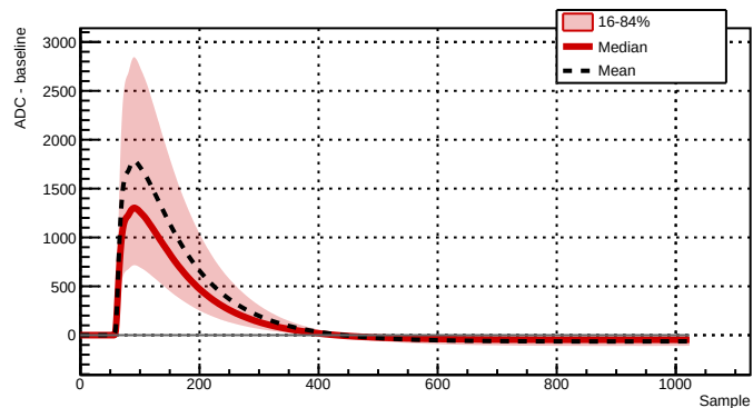
Run 039501 - Channel 2081 - 32436 waveforms
