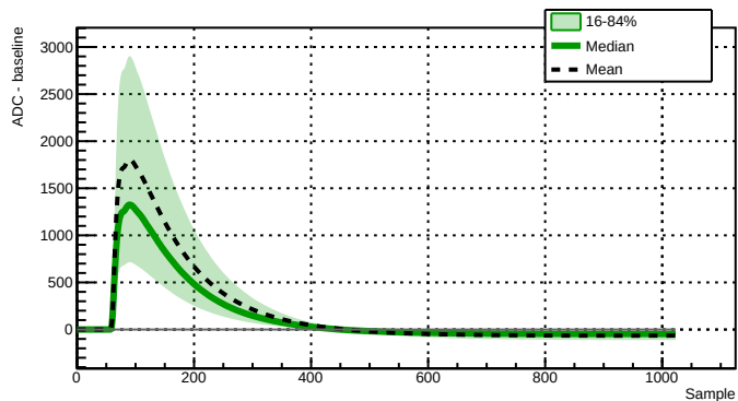
Run 039501 - Channel 2080 - 33111 waveforms
