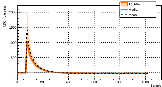
Run 039501 - Channel 2071 - 9232 waveforms
