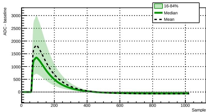
Run 039502 - Channel 2080 - 34159 waveforms
