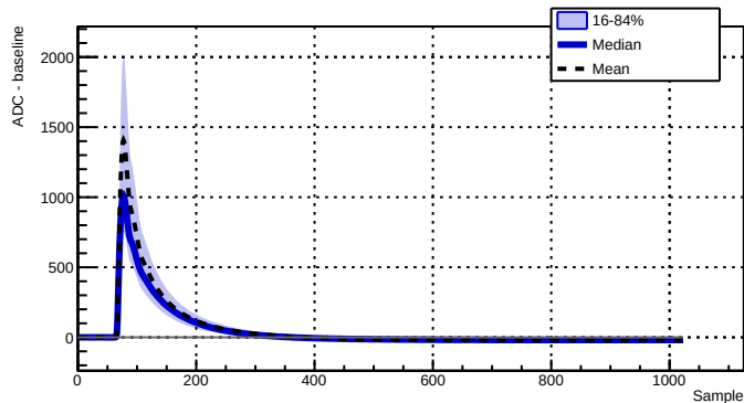
Run 039502 - Channel 2070 - 10286 waveforms
