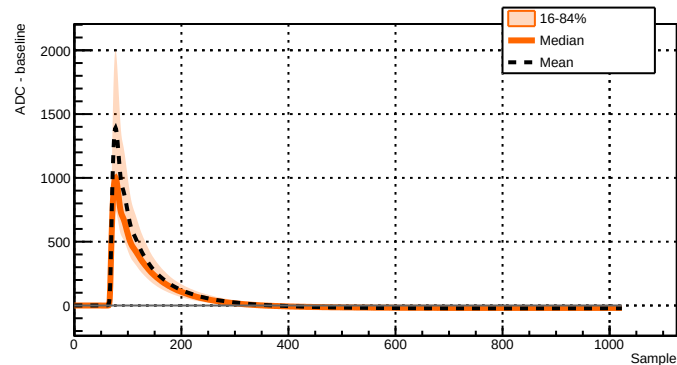
Run 039502 - Channel 2071 - 9912 waveforms
