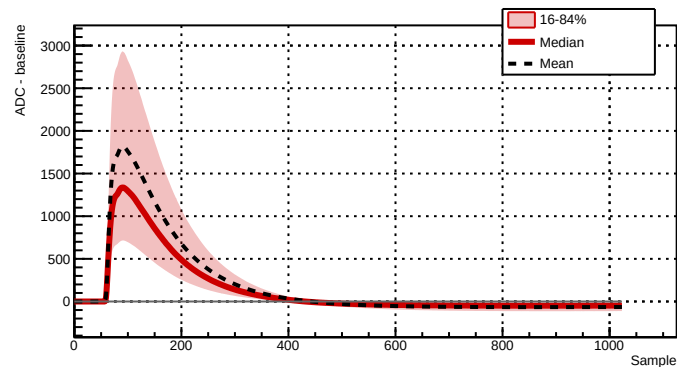
Run 039502 - Channel 2081 - 33406 waveforms
