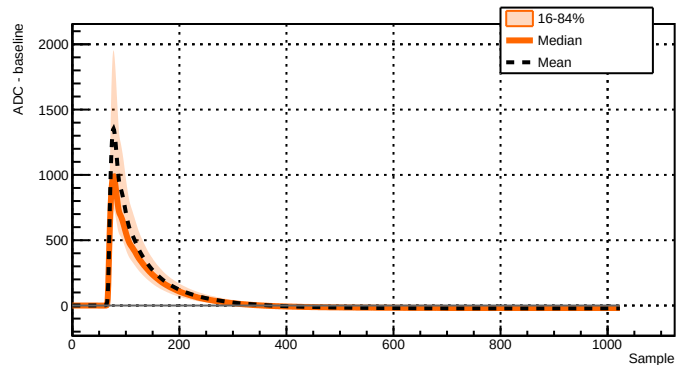
Run 039503 - Channel 2071 - 10874 waveforms
