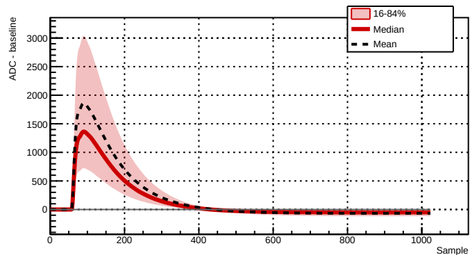
Run 039503 - Channel 2081 - 35420 waveforms
