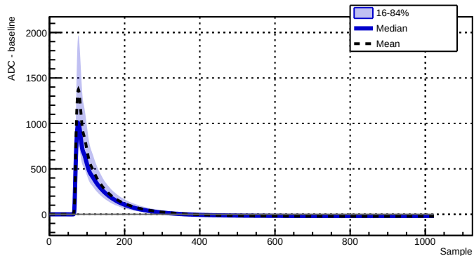
Run 039503 - Channel 2070 - 11234 waveforms
