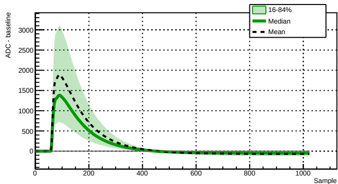
Run 039503 - Channel 2080 - 36104 waveforms
