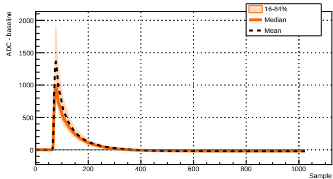
Run 039504 - Channel 2071 - 11469 waveforms
