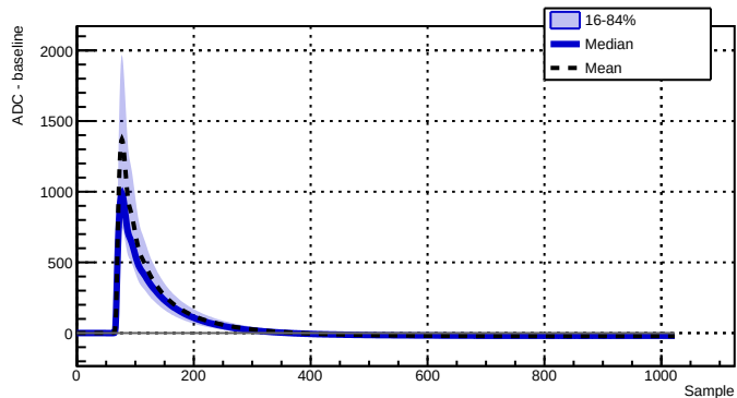
Run 039504 - Channel 2070 - 11853 waveforms
