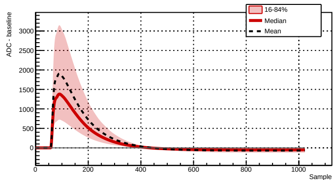
Run 039504 - Channel 2081 - 36788 waveforms
