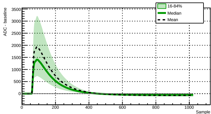
Run 039504 - Channel 2080 - 37342 waveforms
