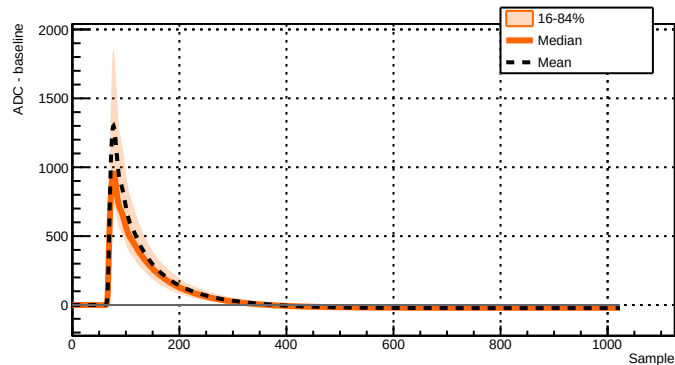
Run 039508 - Channel 2071 - 16016 waveforms
