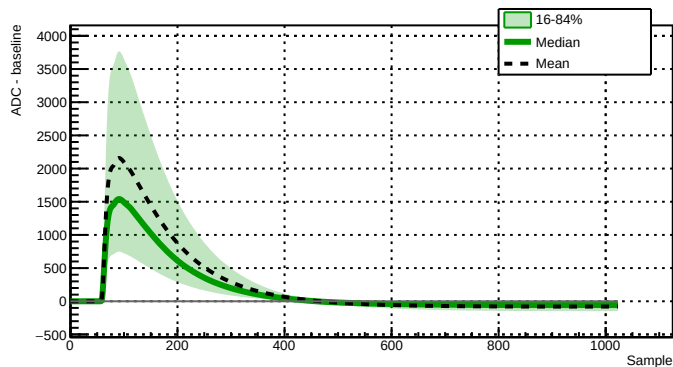
Run 039508 - Channel 2080 - 44256 waveforms
