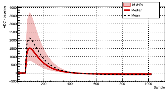
Run 039508 - Channel 2081 - 43629 waveforms
