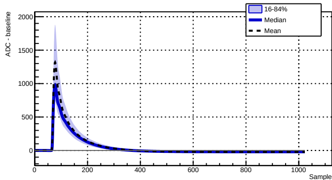
Run 039508 - Channel 2070 - 16558 waveforms
