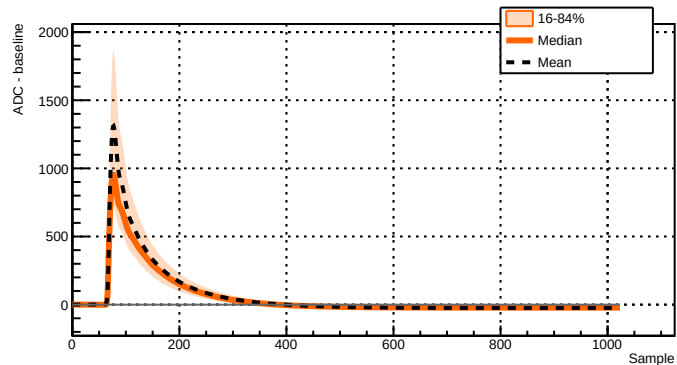
Run 039510 - Channel 2071 - 18503 waveforms
