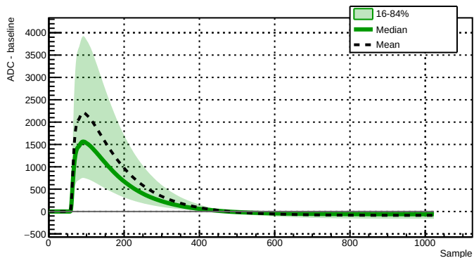
Run 039510 - Channel 2080 - 48059 waveforms
