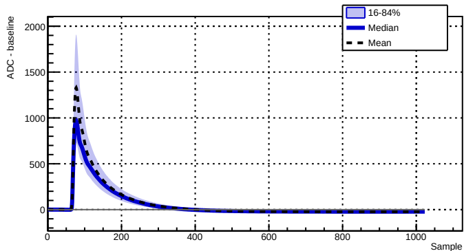
Run 039510 - Channel 2070 - 19057 waveforms
