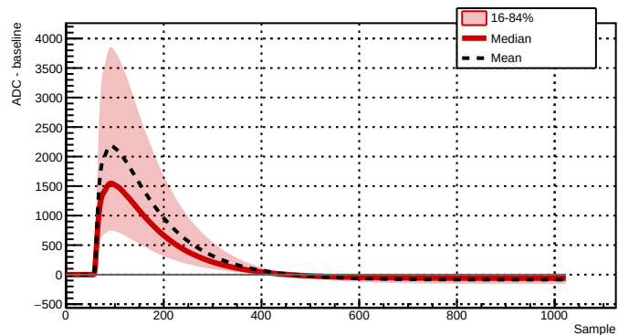
Run 039510 - Channel 2081 - 47507 waveforms
