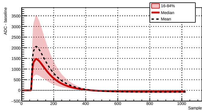
Run 039515 - Channel 2081 - 39804 waveforms
