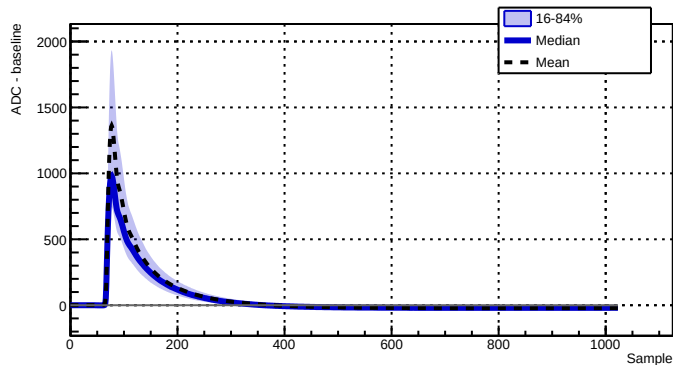
Run 039515 - Channel 2070 - 14412 waveforms
