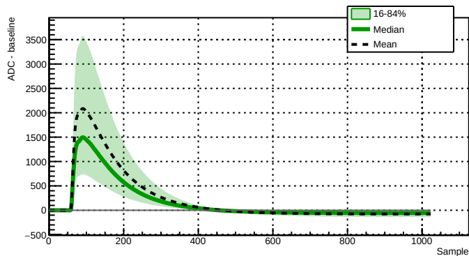
Run 039515 - Channel 2080 - 40436 waveforms
