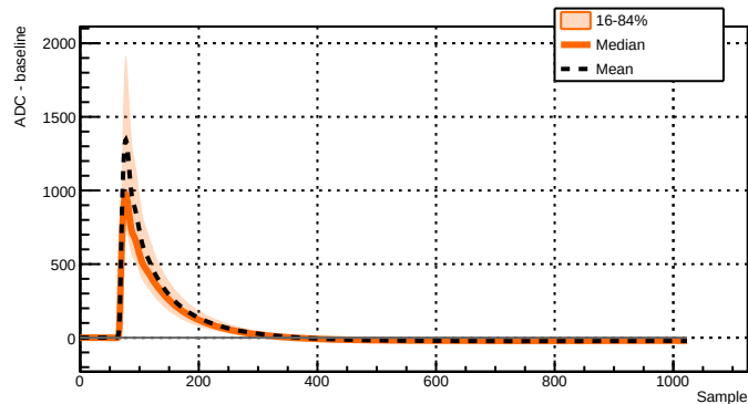
Run 039515 - Channel 2071 - 13922 waveforms
