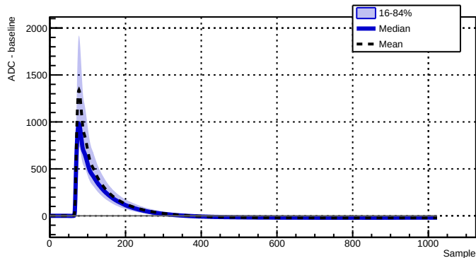
Run 039516 - Channel 2070 - 13440 waveforms
