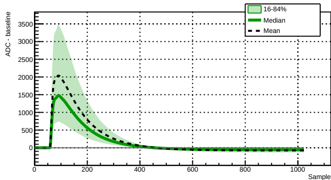
Run 039516 - Channel 2080 - 39237 waveforms
