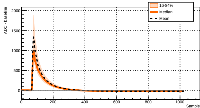
Run 039516 - Channel 2071 - 12969 waveforms
