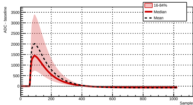
Run 039516 - Channel 2081 - 38693 waveforms
