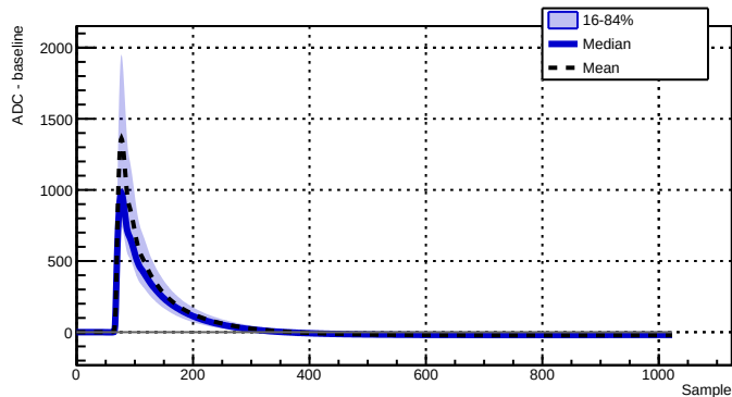
Run 039517 - Channel 2070 - 13126 waveforms
