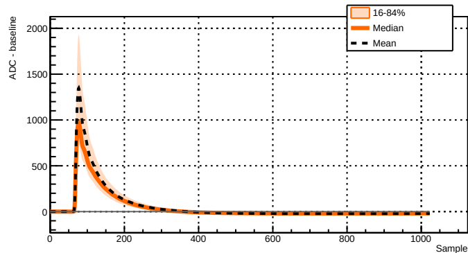
Run 039517 - Channel 2071 - 12700 waveforms
