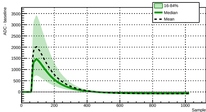
Run 039517 - Channel 2080 - 39067 waveforms
