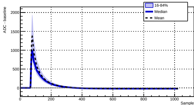
Run 039519 - Channel 2070 - 12009 waveforms
