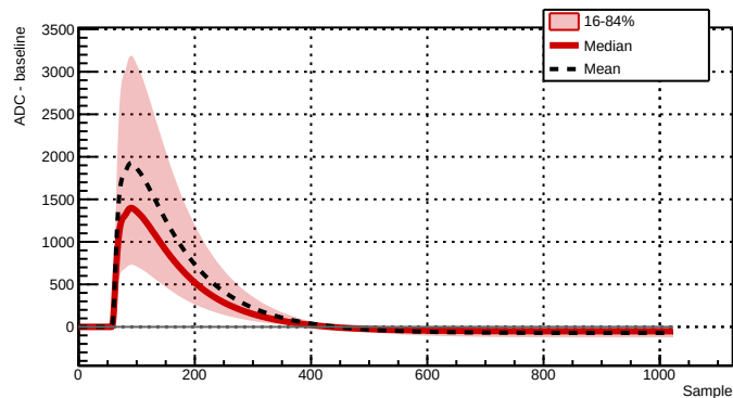
Run 039519 - Channel 2081 - 36497 waveforms
