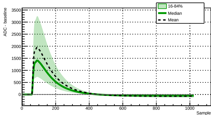
Run 039519 - Channel 2080 - 37265 waveforms
