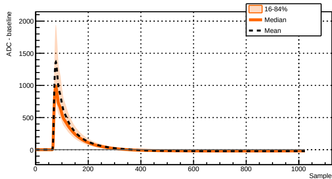
Run 039519 - Channel 2071 - 11455 waveforms
