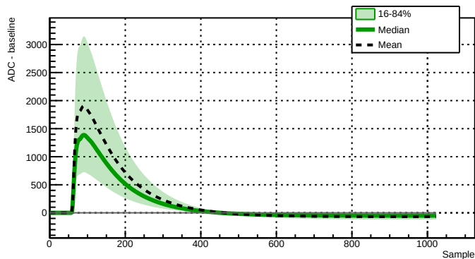
Run 039521 - Channel 2080 - 35947 waveforms
