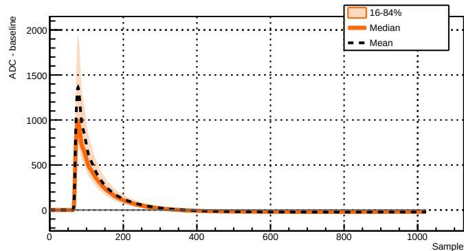
Run 039521 - Channel 2071 - 10859 waveforms
