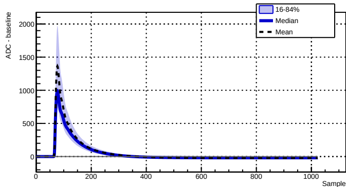
Run 039521 - Channel 2070 - 11337 waveforms
