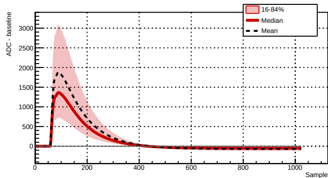
Run 039521 - Channel 2081 - 35297 waveforms
