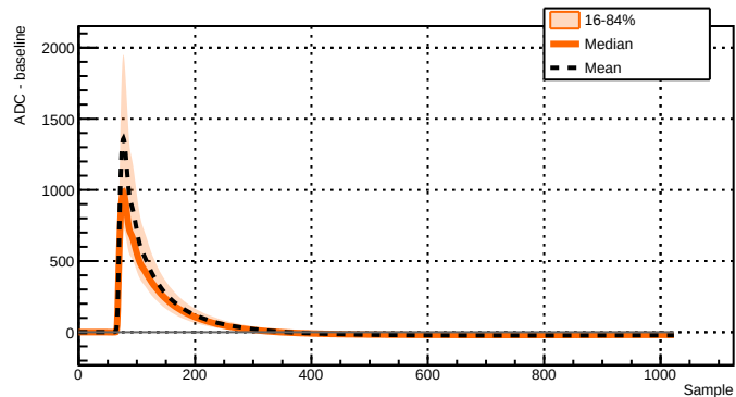
Run 039523 - Channel 2071 - 10027 waveforms
