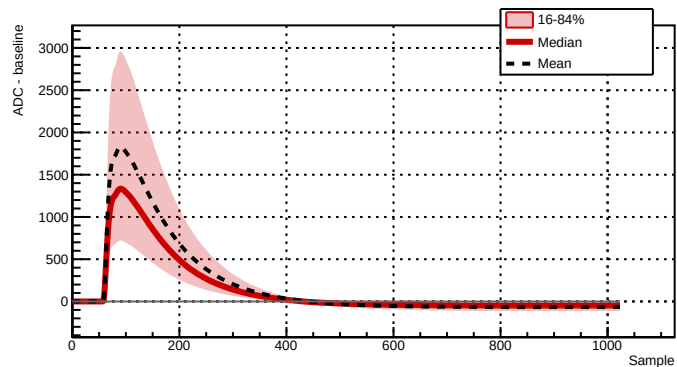
Run 039523 - Channel 2081 - 33759 waveforms
