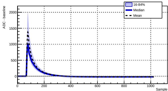
Run 039523 - Channel 2070 - 10377 waveforms
