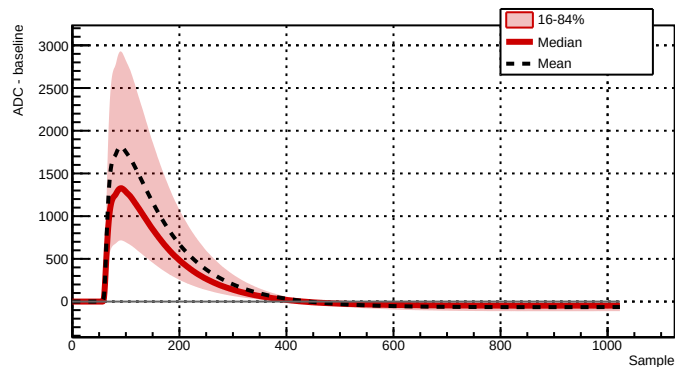
Run 039525 - Channel 2081 - 32792 waveforms
