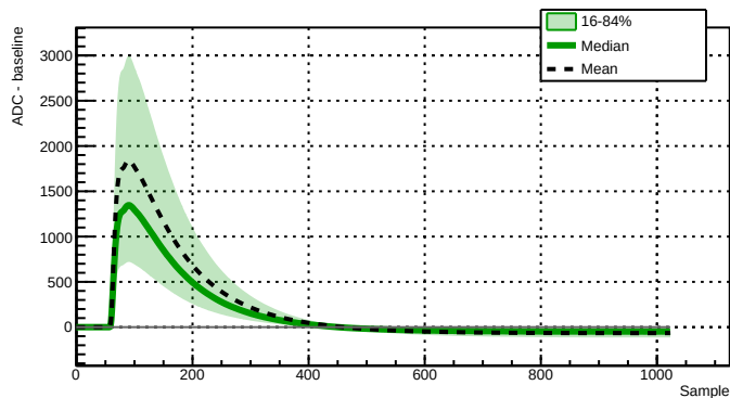
Run 039525 - Channel 2080 - 33381 waveforms
