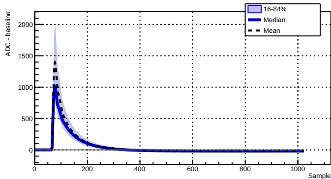
Run 039525 - Channel 2070 - 10069 waveforms
