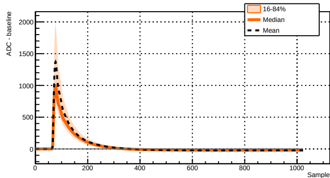
Run 039525 - Channel 2071 - 9793 waveforms
