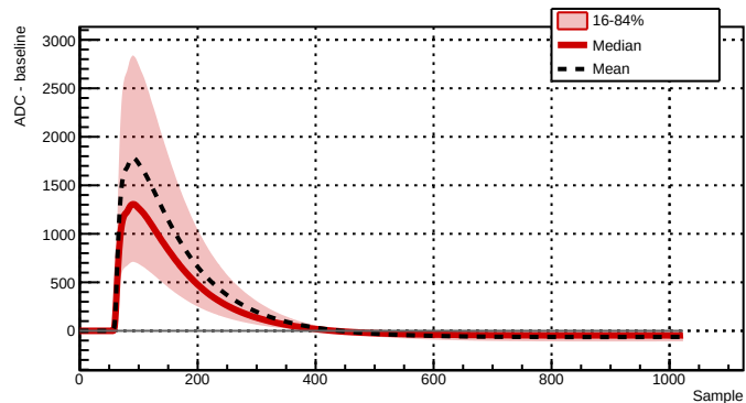
Run 039527 - Channel 2081 - 32008 waveforms
