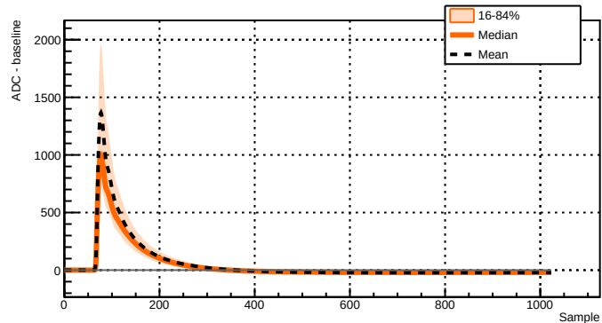
Run 039527 - Channel 2071 - 9208 waveforms
