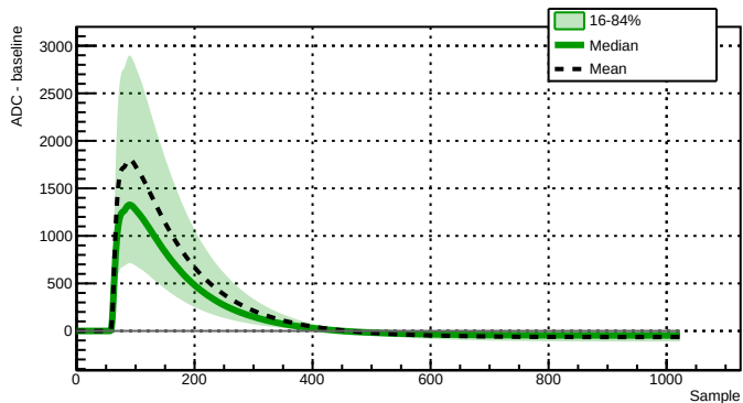
Run 039527 - Channel 2080 - 32743 waveforms
