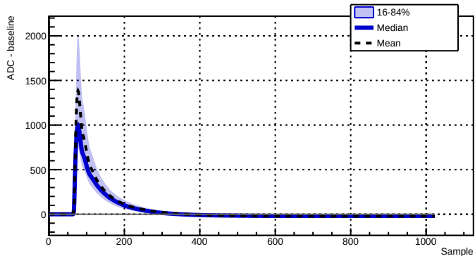
Run 039527 - Channel 2070 - 9515 waveforms
