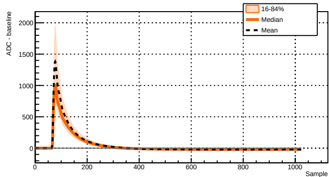
Run 039529 - Channel 2071 - 8725 waveforms
