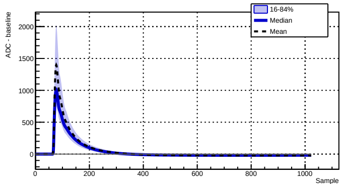
Run 039529 - Channel 2070 - 8946 waveforms
