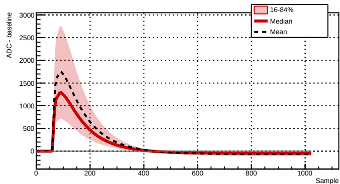
Run 039529 - Channel 2081 - 30916 waveforms
