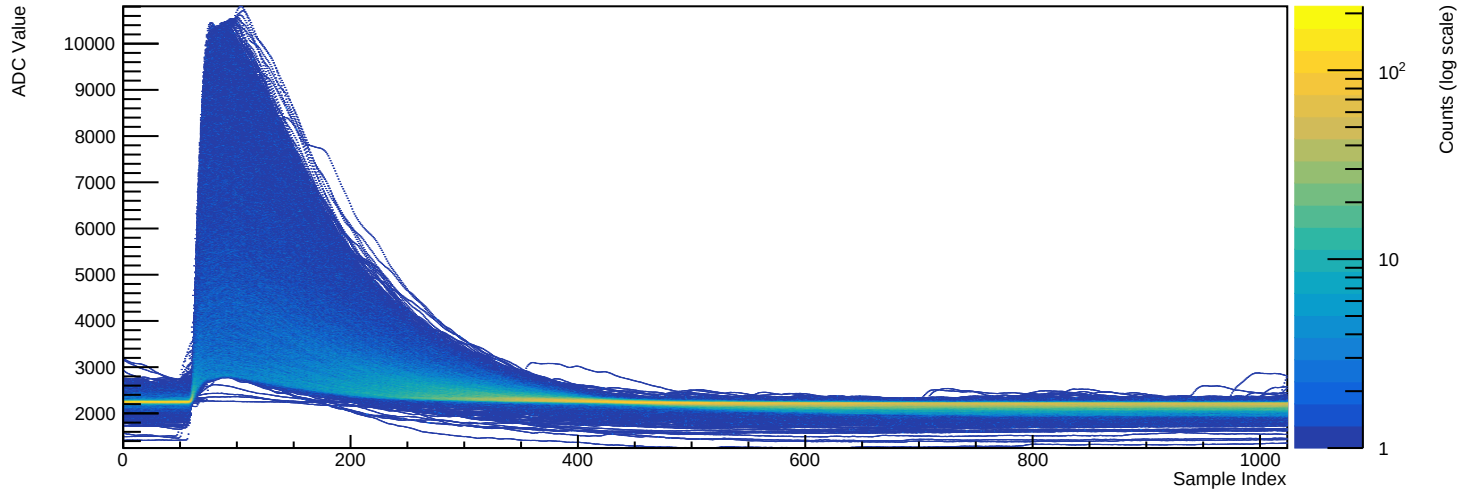
Run 039500 - Channel 2080 (n=6944 waveforms)
