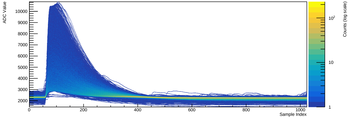
Run 039522 - Channel 2080 (n=7866 waveforms)
