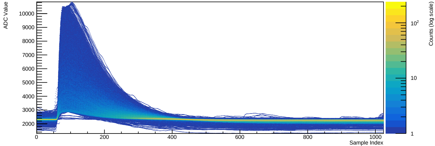
Run 039525 - Channel 2080 (n=7409 waveforms)
