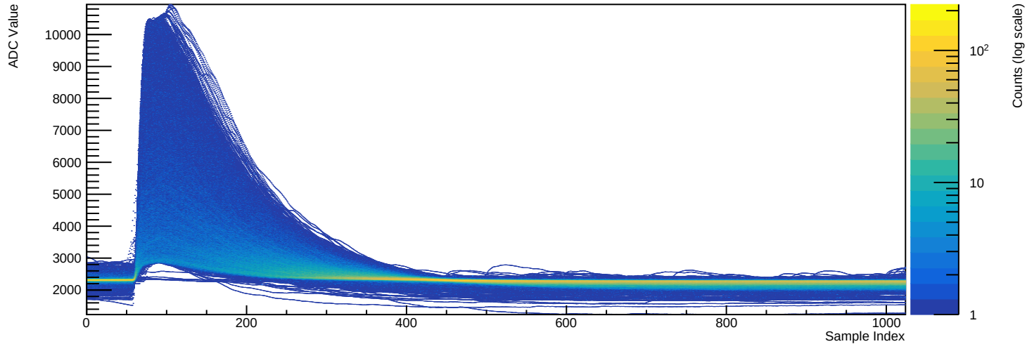
Run 039526 - Channel 2080 (n=7304 waveforms)
