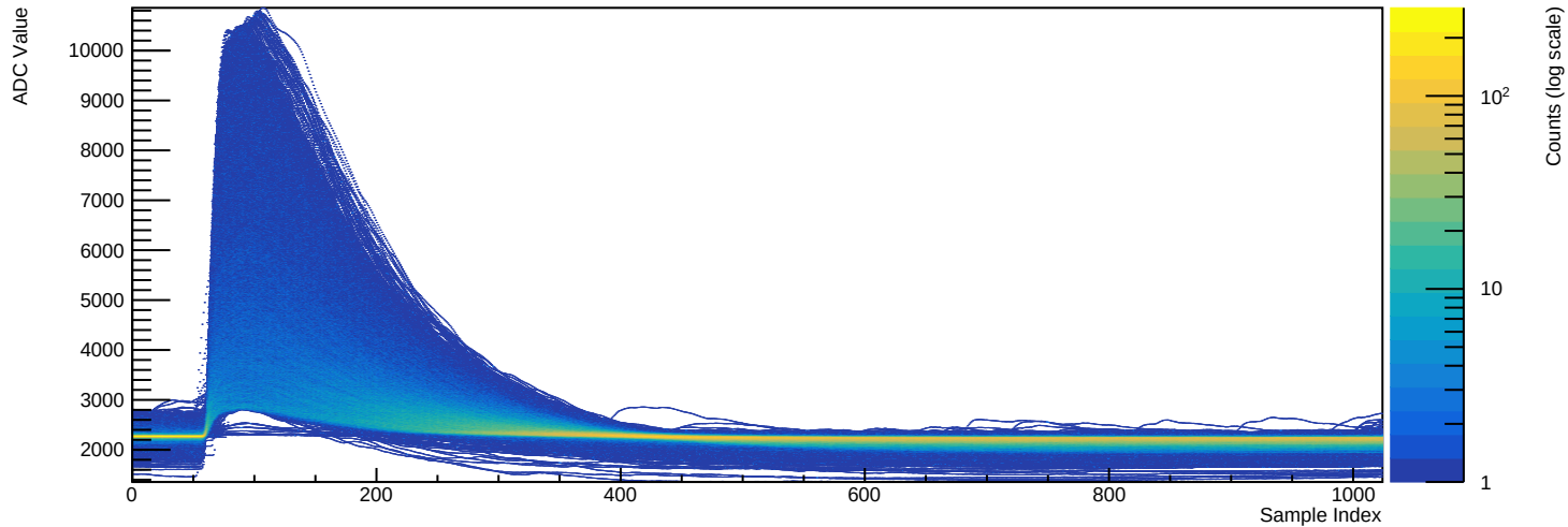
Run 039502 - Channel 2081 (n=9337 waveforms)
