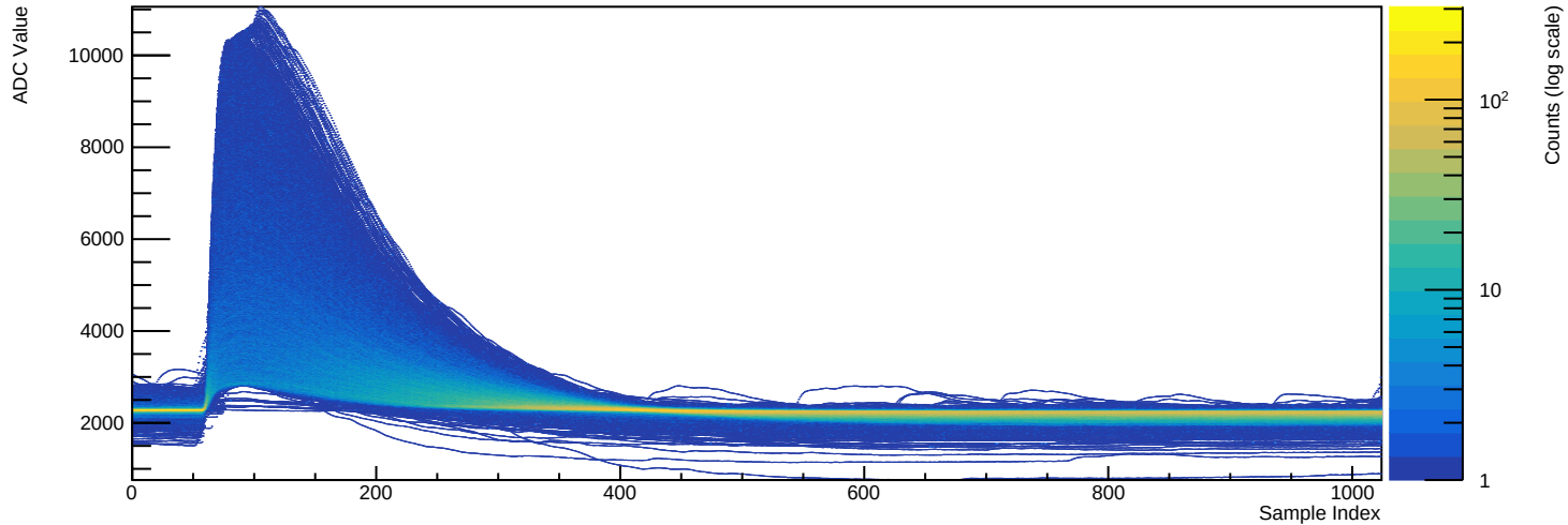
Run 039504 - Channel 2081 (n=10322 waveforms)
