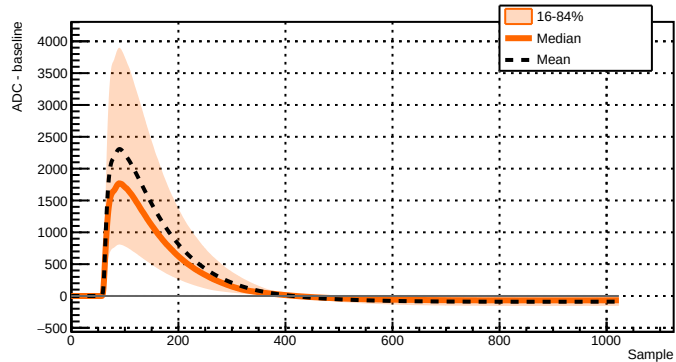
Run 039500 - Channel 2081 - 8788 waveforms
