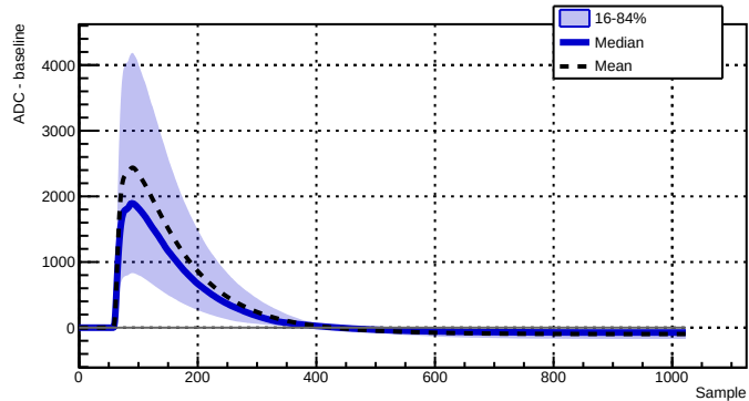
Run 039500 - Channel 2080 - 6944 waveforms
