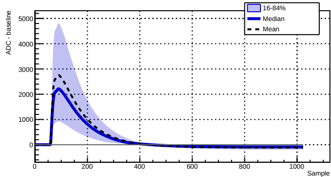
Run 039504 - Channel 2080 - 8106 waveforms
