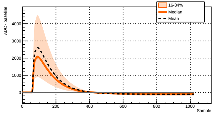
Run 039504 - Channel 2081 - 10322 waveforms
