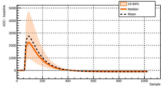
Run 039506 - Channel 2081 - 10921 waveforms
