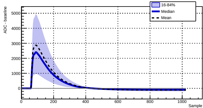
Run 039506 - Channel 2080 - 8671 waveforms
