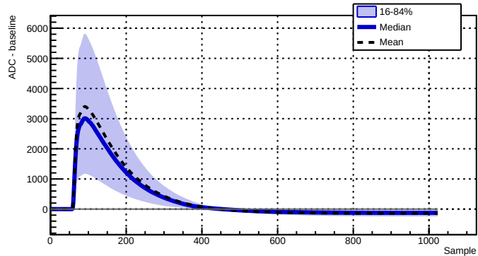
Run 039511 - Channel 2080 - 10016 waveforms
