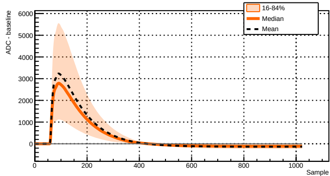
Run 039511 - Channel 2081 - 12237 waveforms
