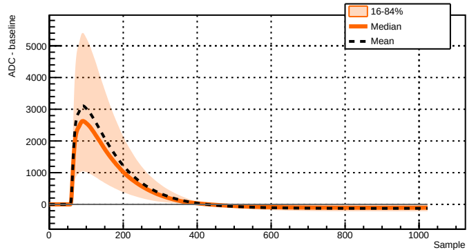
Run 039512 - Channel 2081 - 12170 waveforms
