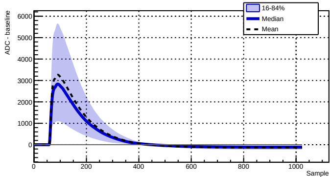
Run 039512 - Channel 2080 - 9816 waveforms
