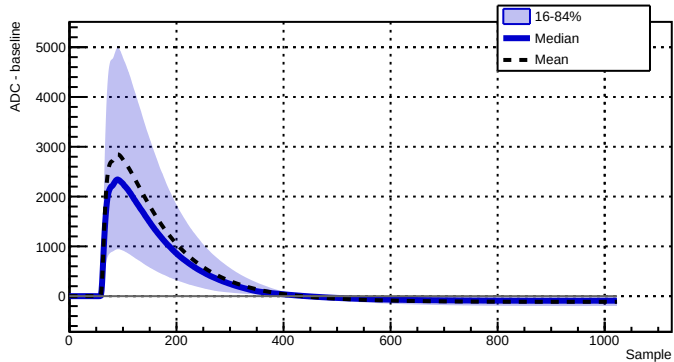
Run 039518 - Channel 2080 - 8491 waveforms
