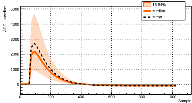
Run 039518 - Channel 2081 - 10543 waveforms
