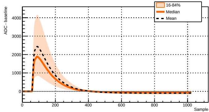
Run 039525 - Channel 2081 - 9035 waveforms
