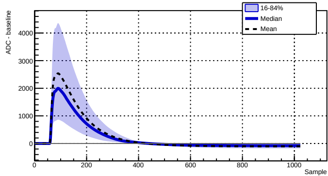
Run 039525 - Channel 2080 - 7409 waveforms
