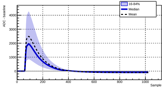
Run 039527 - Channel 2080 - 7271 waveforms
