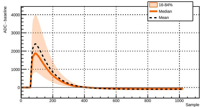
Run 039527 - Channel 2081 - 8947 waveforms
