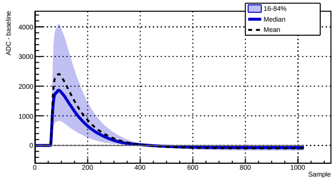
Run 039528 - Channel 2080 - 7142 waveforms
