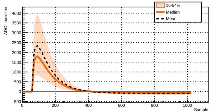
Run 039528 - Channel 2081 - 8681 waveforms
